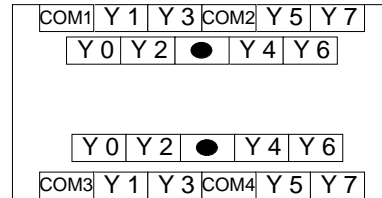
Figure: 2.16 FX0N-8ER-ES/UL
