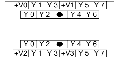
Figure: 2.15 FX0N-16EYT-ESS/UL
